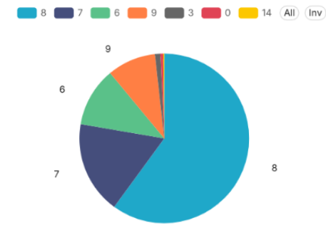
Incident Categories
